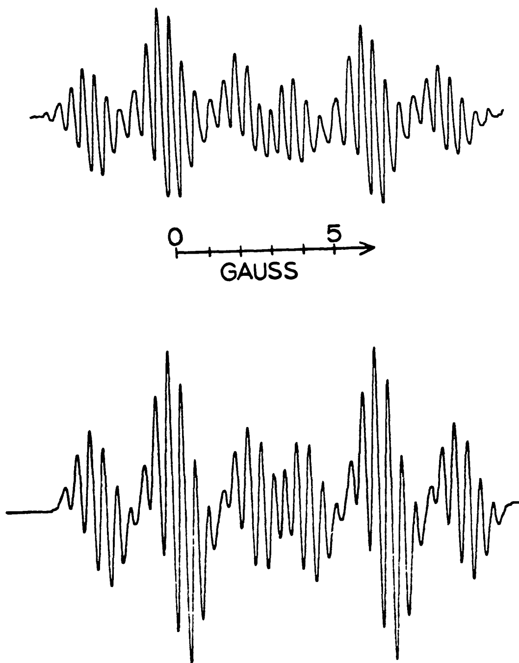
Figure 7. First-derivative esr spectrum of (a) exo, exo -5,6-dideuterobicyclo[2.2.1]heptan-2,3-semidione (VII) prepared by reduction of \alpha -diketone VII-c and, (b) the simulated spectrum using the hfsc of the text.
