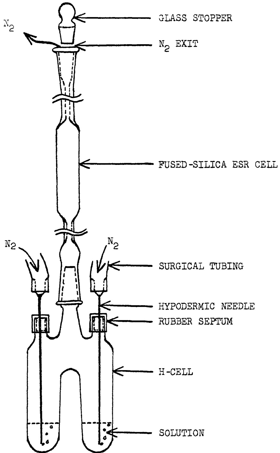
Figure 38. Apparatus for the preparation of solutions of stable radicals.
