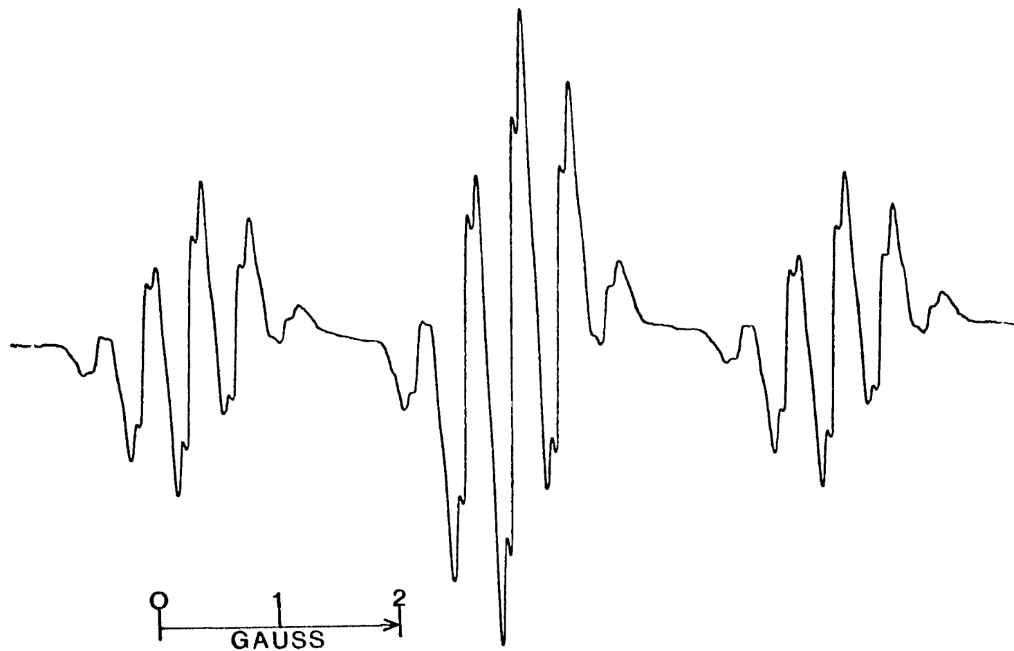
Figure 34. First-derivative esr spectrum of semiquinone I.IV in DMSO.
