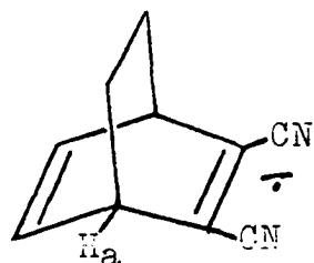
LXXIII a_{H_a}^H = 0.225
