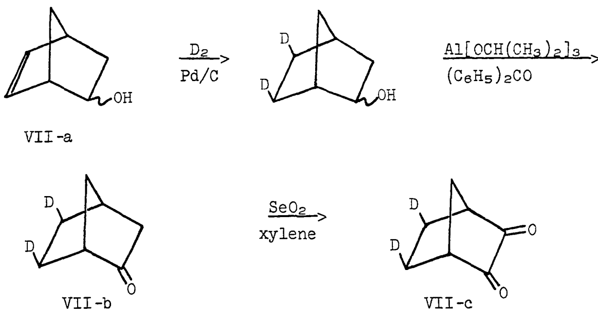
Scheme II
