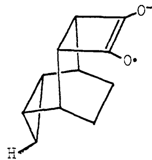
XLVI a^{\text{H}} = 0.68
