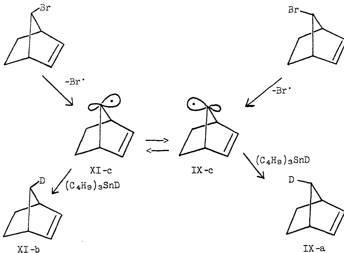
Scheme IX
