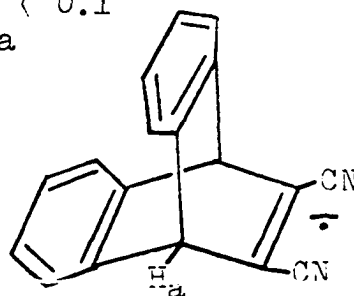
LXXIV a_{H_a}^H = 0.15
