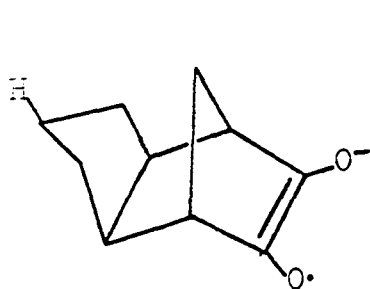
XIX a^{\text{H}} = 1.31
