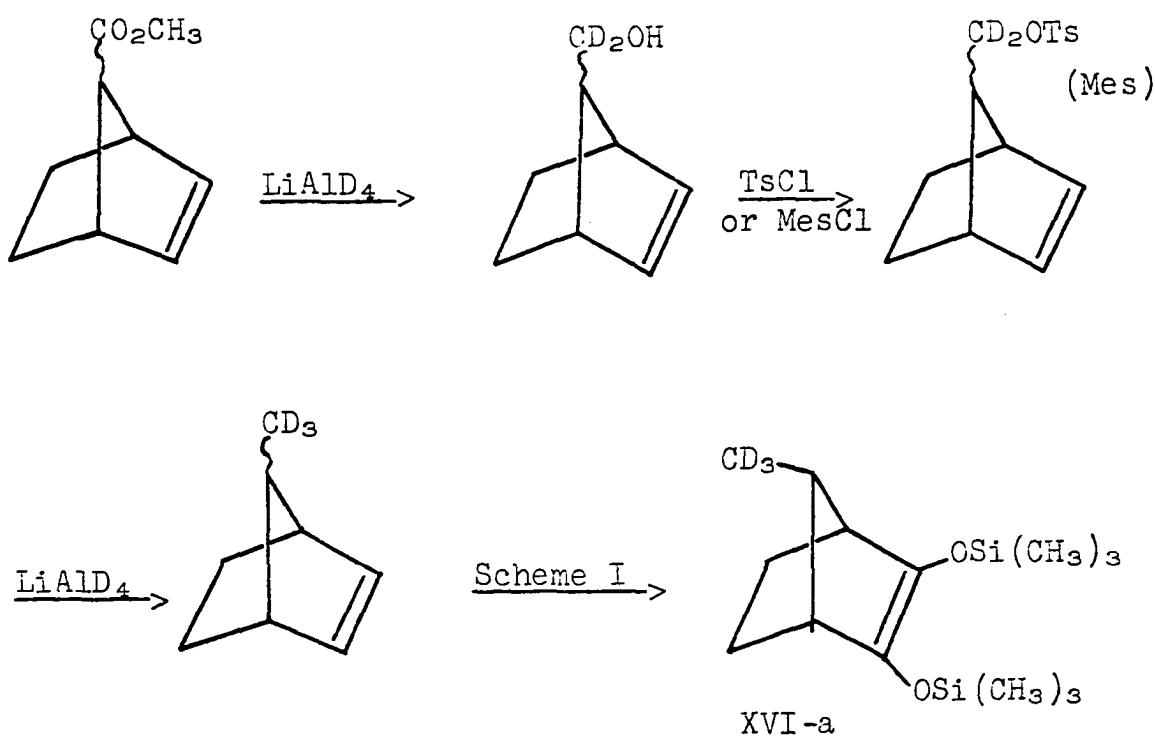
Scheme III
