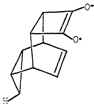
XLV a^{\text{H}} = 1.06
